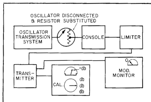
Fig. 1. Carrier hum and noise setup.
