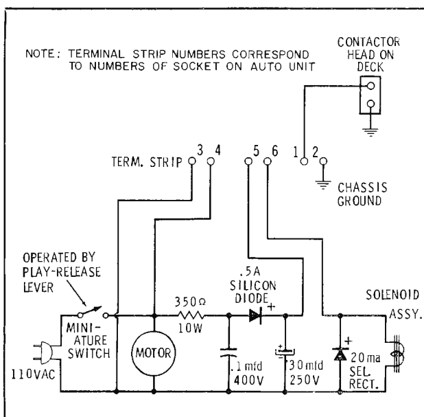
Fig. 2. Modified circuit of the cartridge-tape transport.
